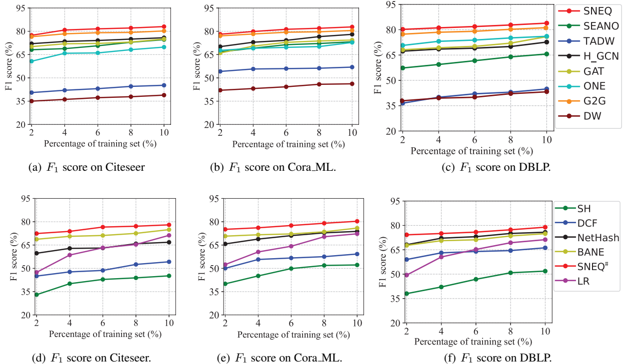
Figure 2: Node classification results on the three attributed networks. The top row shows the results of continuous embeddings while the bottom row shows the results of discrete embedding results.
