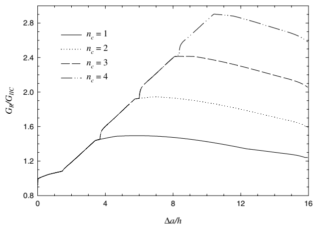
Fig. 10. Influence of number of z-pin columns, n_c , on normalized delamination toughness, G_R/G_{IIC} , during crack growth with T_d/G_{IIC}h = 190.5 , \delta_a/h = 0.00667 and d_c/h = 2.33 .
