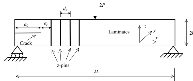
Fig. 1. Illustration of a mode II delamination test for z-pin reinforced laminate: end-notched-flexure (ENF) geometry.
