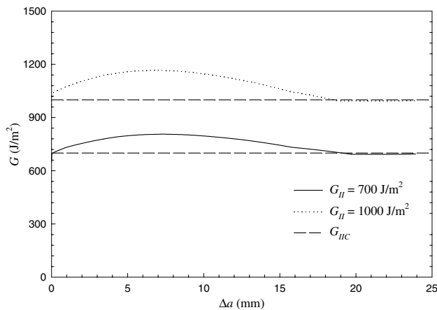
Fig. 6. Calculated energy release rate G of an unpinned ENF specimen as a function of crack growth \Delta a for different critical energy release rates, G_{II} = 700 and 1000 J/m 2 .
