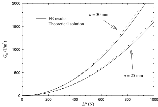
Fig. 5. Variation of mode II energy release rate G_{II} versus applied force 2P for a = 25 and 30 mm.
