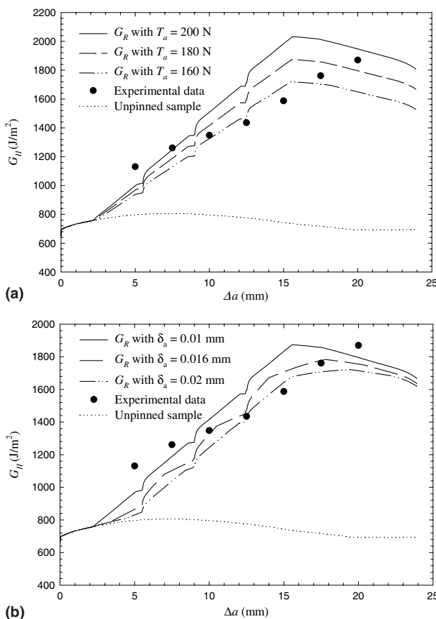
Fig. 7. (a) Predicted crack-resistance G_R curves of z-pinned ENF laminates versus crack growth \Delta a for different values of T_a while keeping constant \delta_a of 0.01mm, compared to experimental data and an unpinned sample ( G_{IIC} = 700 J/m 2 ). (b) Predicted crack-resistance G_R curves of z-pinned ENF laminates versus crack growth \Delta a for different values of \delta_a while keeping constant T_a of 180 N, compared to experimental data and an unpinned sample ( G_{IIC} = 700 J/m 2 ).
