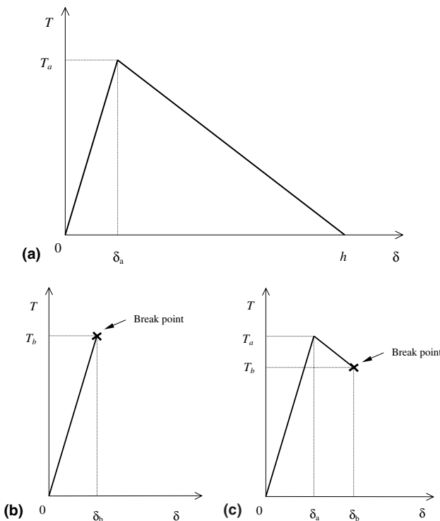
Fig. 3. (a) Schematic of mode II z-pin pullout model with pin completely pulled out, which is assumed in this study. (b) Schematic of mode II z-pin pullout model with pin breakage at the peak pullout force. (c) Schematic of mode II z-pin pullout model with pin breakage after reaching the peak pullout force.
