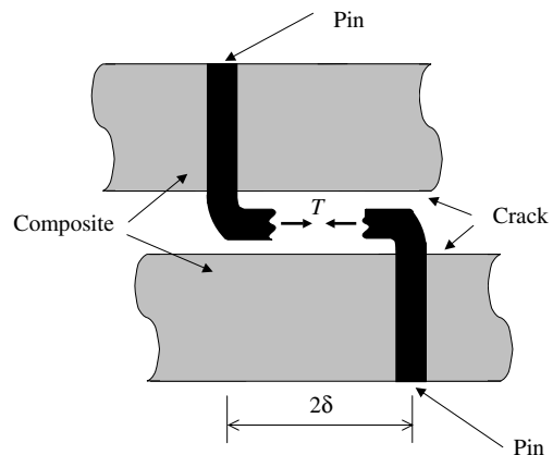
Fig. 2. Schematic of the pullout of a z -pin under mode II delamination.
