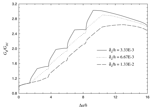
Fig. 8. Influence of normalized pullout model parameter, \delta_a/h , on normalized delamination toughness, G_R/G_{IIC} , during crack growth with n_c = 4 , T_a/G_{IIC}h = 190.5 and d_c/h = 2.33 .
