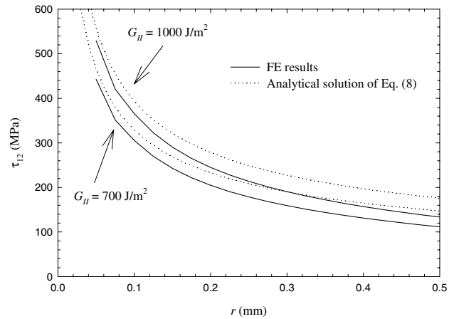
Fig. 4. The variation of shear stress, \tau_{12} , ahead of the crack-tip with applied energy release rates G_{II} = 700 and 1000 \text{ J/m}^2 , respectively.
