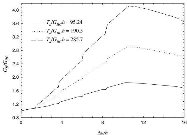
Fig. 9. Influence of normalized pullout model parameter, T_d/G_{IIC}h , on normalized delamination toughness, G_R/G_{IIC} , during crack growth with n_c = 4 , \delta_a/h = 0.00667 and d_c/h = 2.33 .
