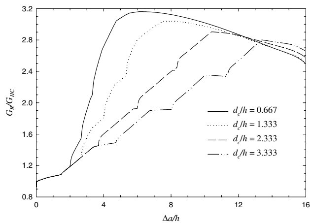
Fig. 11. Influence of normalized column spacing, d_c/h , on normalized delamination toughness, G_R/G_{IIC} , during crack growth with T_d/G_{IIC}h = 190.5 , \delta_a/h = 0.00667 and n_c = 4 .
