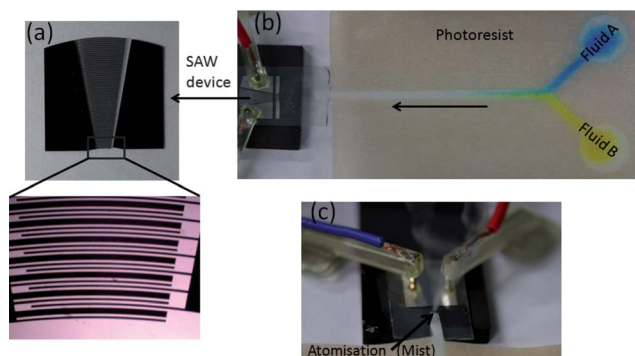
Fig. 2 (a) Image of the focused SPUDT across which an oscillating RF signal is applied to generate the SAWs that act to draw flow through the paper microfluidics device. (b) The end of the flow channel at the edge of the paper is placed at the focal point of the SAW such that (c) the atomisation of the fluid out of the channel at the paper edge draws liquid through the Y-channel from its two reservoirs.
