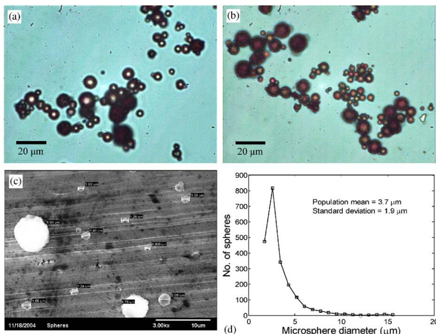
Fig. 3. Microspheres produced by the AC electrospay. (a) DI water encapsulated within microspheres; (b) DI water and uranine dye encapsulated within microspheres; (c) SEM micrograph of 1–10 \mu\text{m} biodegradable microspheres; (d) size distribution of the microspheres. Although the visual method of size characterization in (d) could only account for microspheres above 1 \mu\text{m} , the SEM image in (c) and those shown subsequently indicate that sub-micron particles are present in abundance.
