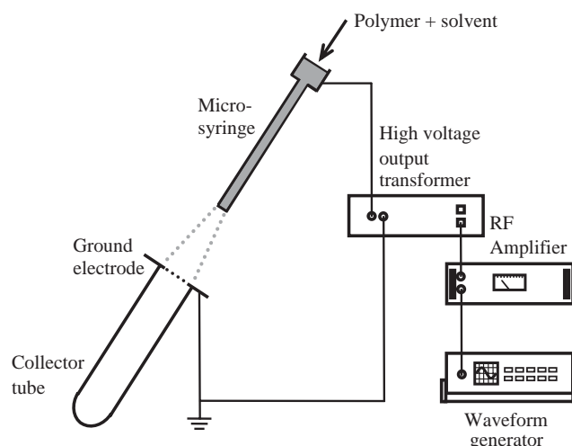
Fig. 1. Schematic of the AC electro-spray apparatus used for microencapsulation and fiber synthesis.
