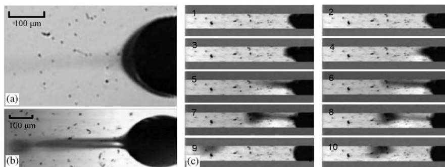
Fig. 2. AC electro spray drop ejection mechanisms. (a) Drop ejection due to viscous pinch-off (tip streaming); (b) drop ejection due to inertial pinch-off resulting in microjet formation; (c) sequences of images at 6000 frames/s showing the development of the microjet and subsequent drop detachment.
