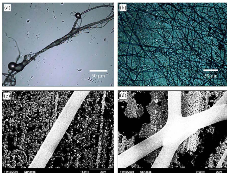
Fig. 4. AC electrospay fiber synthesis. (a) A 10 \mu\text{m} compound fiber. (b) A network of 1 \mu\text{m} single strand fibers produced by the AC electrospay. SEM images of (c) a single-strand fiber, and (d) a network junction of single strand fibers. Both (c) and (d) are magnified from the fiber mesh network in (b). The compound fiber in (a) consists of an entanglement of sub-micron fiber strands. In (c) and (d), the background shows submicron polymer particles similar to those obtained in Fig. 3c, obtained concurrently with the fiber synthesis.
