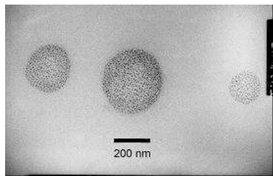
Figure 5. Transmission electron microscopy of the particles obtained by SAW atomization and solvent evaporation.
