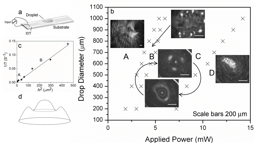
Figure 1. (a) Schematic depiction of the experimental setup. (b) Interfacial colloidal patterns as a function of the initial drop diameter and input power. (c) Inverse particle clustering time as a function of the square of the amplitude of the standing wave. (d) Circular nodal ring arising from large amplitude vibration of the drop interface at the capillary-viscous resonant frequency.
