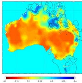
Figure 4: Map of the LAPS soil moisture on 6 January, 2005. The black lines are 20 mm precipitation contours from the previous 24 hours, and the resolution is 0.375°.
