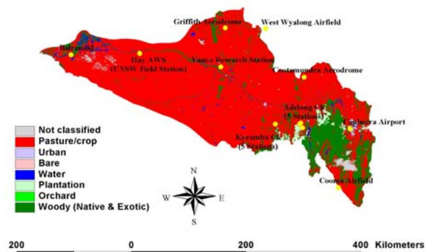
Figure 1: The Murrumbidgee River basin. The ten Murrumbidgee Soil Moisture Monitoring Network station locations used in this study are marked in yellow; the overlay is land-cover.
