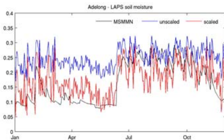
Figure 5: Comparison of the LAPS soil moisture to MSMMN data for 2005, at Adelong.
