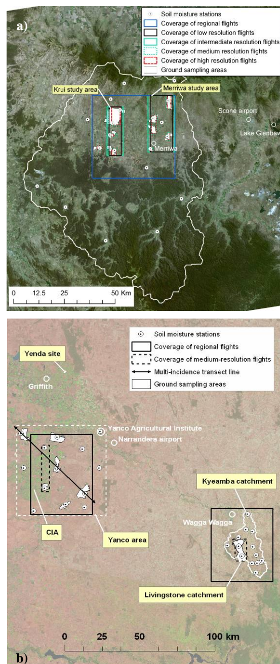
Figure 3. Maps showing location of the study sites, flight coverages and focus farms for ground sampling in a) NAFE'05 and b) NAFE'06.
