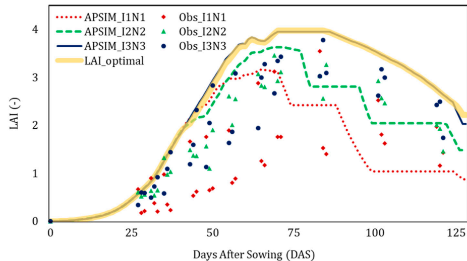
Figure 7. Simulated (APSIM) and observed (Obs) temporal LAI of different treatment plots.
