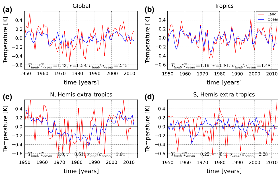
Fig. 2 Observational annual mean T_{land} and T_{ocean} using detrended HadSST2 and CruTEMP4 data
