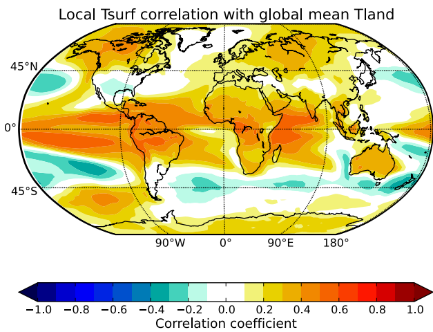
Fig. 4 Correlation between T_{surf} at each grid point and globally averaged timeseries of T_{land} . Data is the annual mean temperature anomalies from 35 CMIP5 pre-industrial control runs, 100 years from each model combined end-to-end to generate a 3,500 year timeseries
