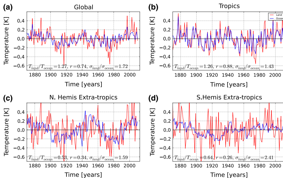
Fig. 5 Annual mean T_{land} and T_{ocean} for a global, b tropical, c Northern Hemisphere extra-tropical, d Southern Hemisphere extra-tropical. Detrended AMIP run forced with HadISST
