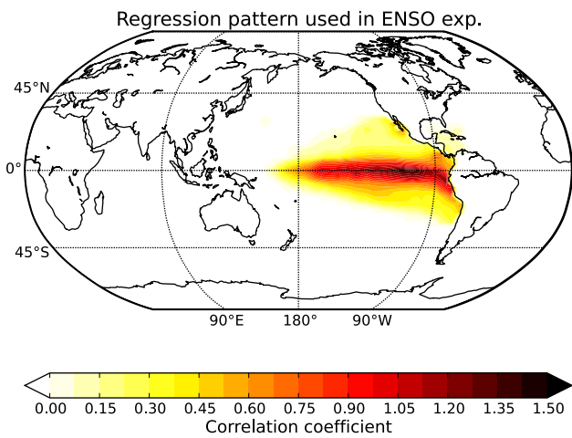
Fig. 1 Pattern used in ENSO experiments. Result of regression between NINO3 and global SST
