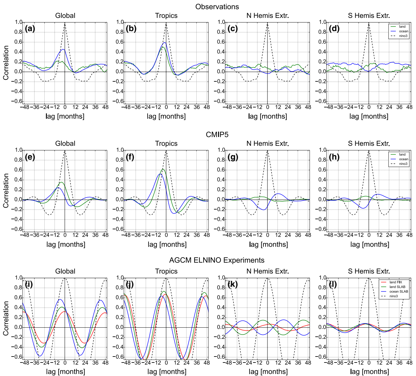
Fig. 8 Cross-correlations between the NINO3 region and land and ocean. Observations ( top row ), combined CMIP5 models ( middle row ), two sensitivity experiments ( bottom row ); atmospheric model forced with ENSO-like oscillation in tropical Pacific and fixed SSTs elsewhere ( red line ), slab ocean elsewhere ( green, blue lines ). Global
