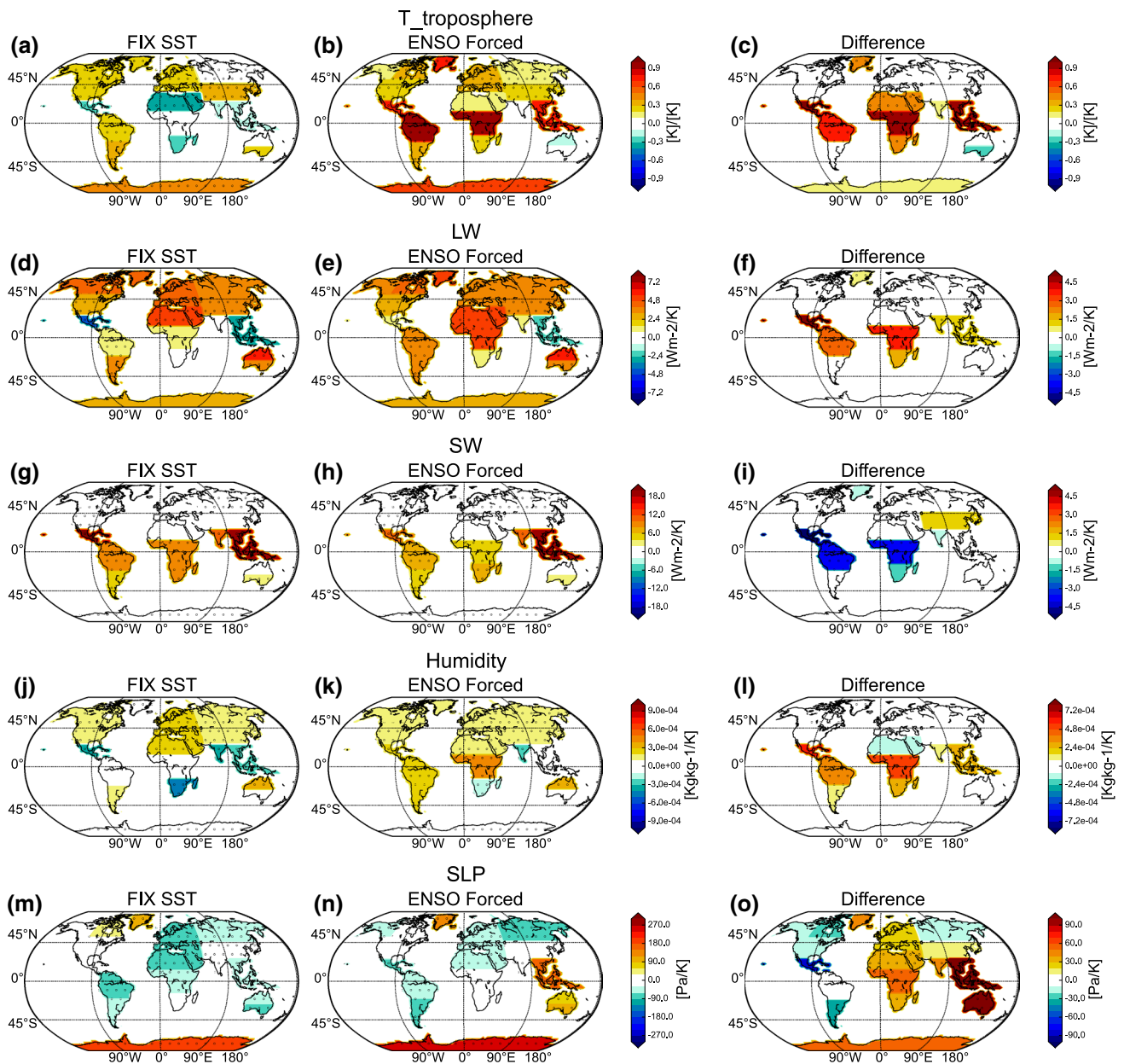
Fig. 10 Regression values between surface and variable averaged over regions. Control run ( left ), forced run ( middle ), difference ( right ). a–c Upper tropospheric temperature (500–100 hPa), d–f
