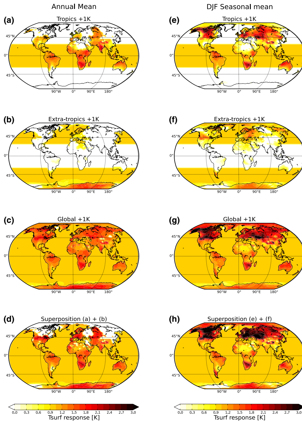
Fig. 7 Mean T_{surf} response for sensitivity experiments, a 1 K added to tropical oceans, b 1 K added to extra-tropical oceans, c 1 K added to global oceans, d combined response of tropical 1 K oceans plus extra-tropical 1 K ocean. Masked at 95 % confidence levels
