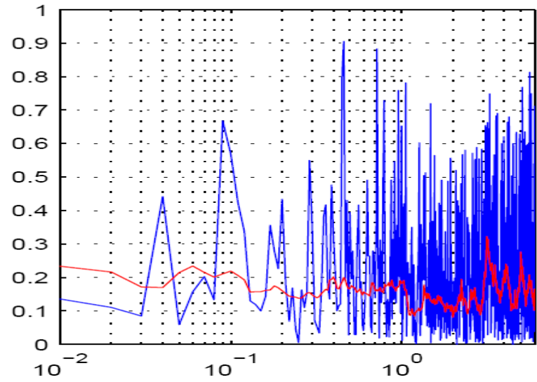
a) Coherence: Northern vs. Southern Pacific
