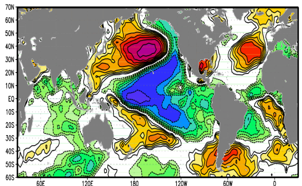
b) ECHAM-OZ no ocean dynamics (EOF-1; 29%)
