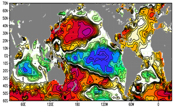
a) Observed (EOF-1; 32%)
