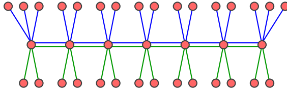
FIGURE 2. Covering a degree-6 caterpillar by two degree-4 subtrees.
