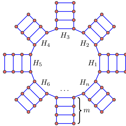
FIGURE 4. Construction in the proof of Proposition 9.7.
