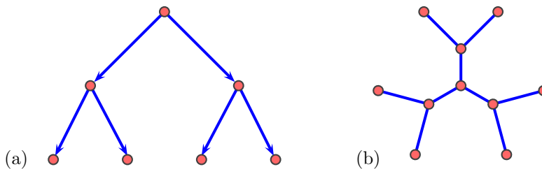
FIGURE 1. (a) \vec{\Gamma}_{2,2} and (b) \Gamma_{3,2} .
