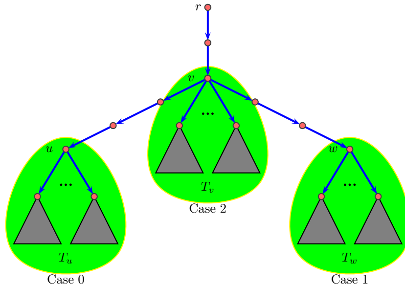
FIGURE 3. Construction in the proof of the upper bound in Theorem 7.1.
