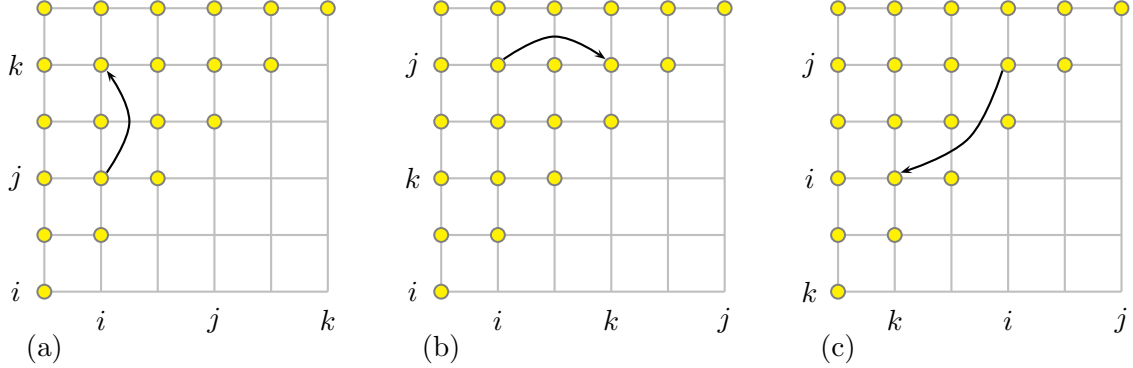
FIGURE 1. Construction of the oriented graph D .
