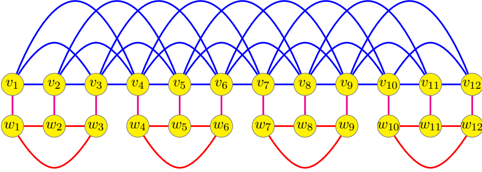
Fig. 4. The construction in Theorem 20 with k = 3 and n = 2 .
