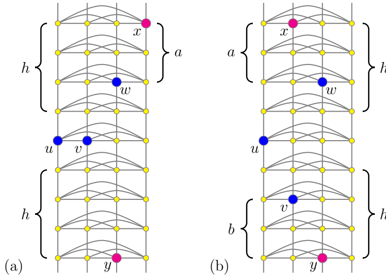
Fig. 3. Illustration for Theorem 16.
