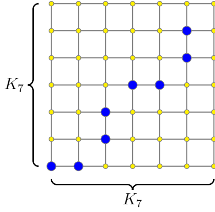
Fig. 2. Resolving set of K_7 \square K_7 with one empty row, one empty column, and no lonely vertex.
