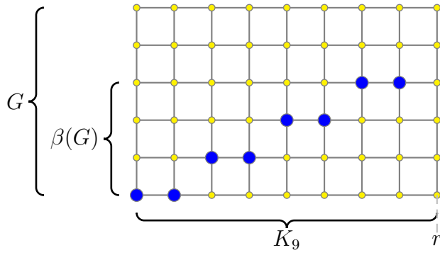
Fig. 1. The resolving set T of K_9 \square G in Lemma 6.
