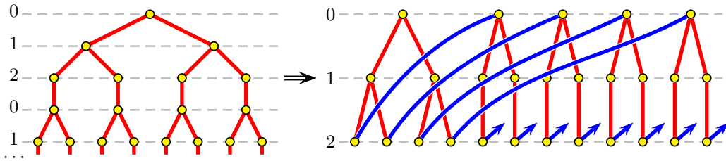
Figure 2: A 3-track layout of T .
