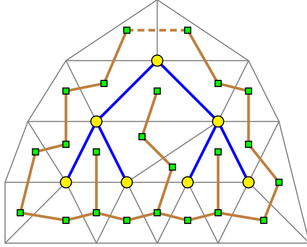
Figure 1: Construction of H in Lemma 8.
