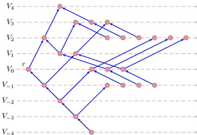
Figure 5 An upward track layout of a tree dag with span 2.
