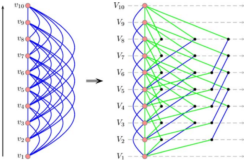
Figure 7 (2, n) -track layout in the proof of Theorem 10.1.
