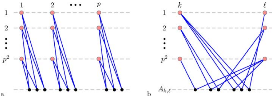
Figure 3 Construction of a track layout of K'_n .
