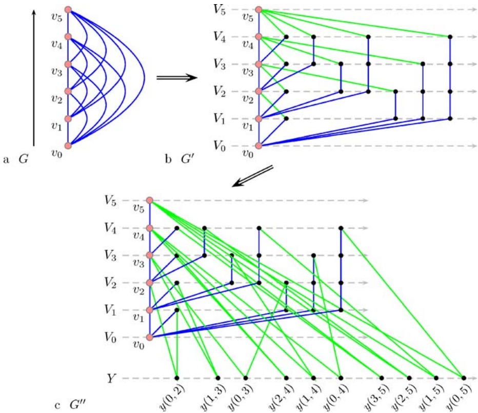
Figure 8 Track layouts in the proof of Theorem 10.2.
