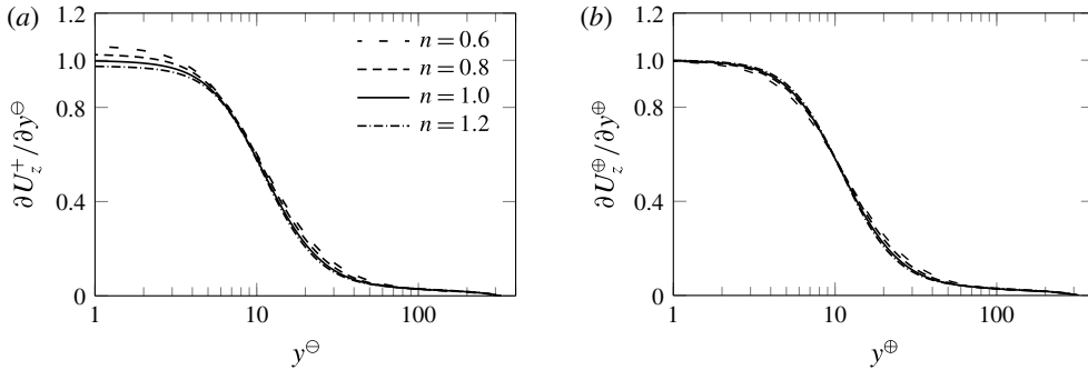
FIGURE 12. Profiles of the mean axial velocity gradient for different n where the non-dimensionalisation used (a) u^* for the velocity scale and the mean wall viscosity \bar{\nu}_w for the viscosity scale, (b) u^\# for the velocity scale and \bar{\nu}_w for the viscosity scale.
