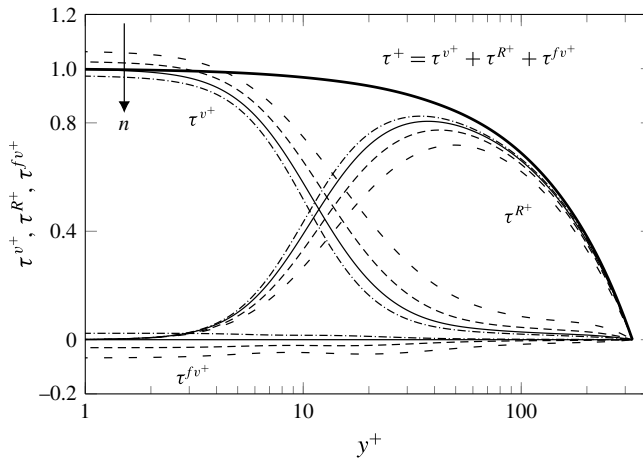
FIGURE 10. Profiles of the (r, z) component of the mean viscous stress, \tau^{v+} , Reynolds shear stress, \tau^{R+} , and the turbulent viscous stress, \tau^{fv+} , plotted for different n . The profile of the total mean stress \tau^+ is linear and the same for all n and is given by (4.1).
