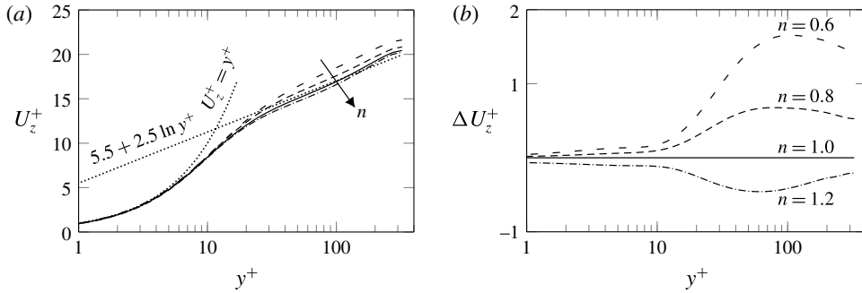
FIGURE 8. Profiles of (a) mean axial velocity U_z^+ and (b) difference between U_z^+ for a PL and Newtonian fluid plotted against y^+ .
