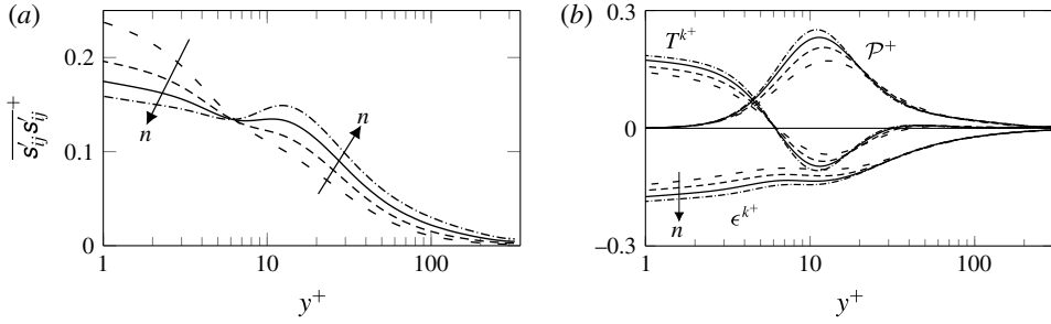
FIGURE 22. Profiles of (a) \overline{s'_{ij}s'_{ij}}^+ (b) turbulent kinetic energy production ( \mathcal{P}^+ ), total dissipation ( \epsilon^{k^+} = \epsilon^+ + \chi_{nn}^+ + \epsilon_{nn}^+ ) and transport ( T^k^+ = \mathcal{T}^+ + \Pi^+ + D^+ + D_{nn}^+ + \xi_{nn}^+ ) plotted in wall units.
