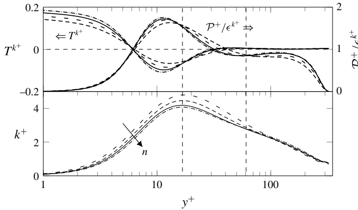
FIGURE 23. Profiles of the ratio of turbulent kinetic energy production to total dissipation ( \mathcal{P}^+/\epsilon^{k+} ), total transport ( T^{k+} ) and the turbulent kinetic energy k^+ plotted in wall units.
