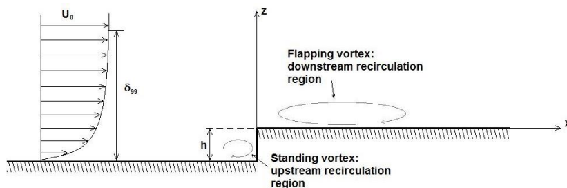
Figure 1. Diagram of forward facing step.
