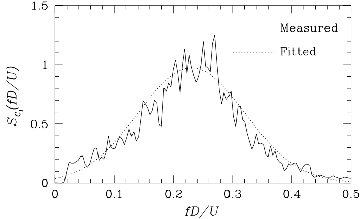
FIGURE 12. Turbulence config. 4: spectrum of lift force recorded at one of the central transducers at Re = 4.95 \times 10^5 . Also shown for comparison is a fitted spectrum of the form given by eq. (4.2). Measured value of C'_l = 0.46 ; fitted value 0.47.
