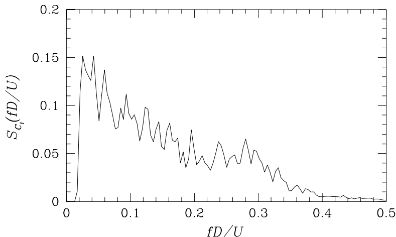
FIGURE 10. Spectrum of lift near the upper end of the Reynolds number range for turbulence config. 2. (Compare fig. 8 G.) Re = 5.37 \times 10^5 .
