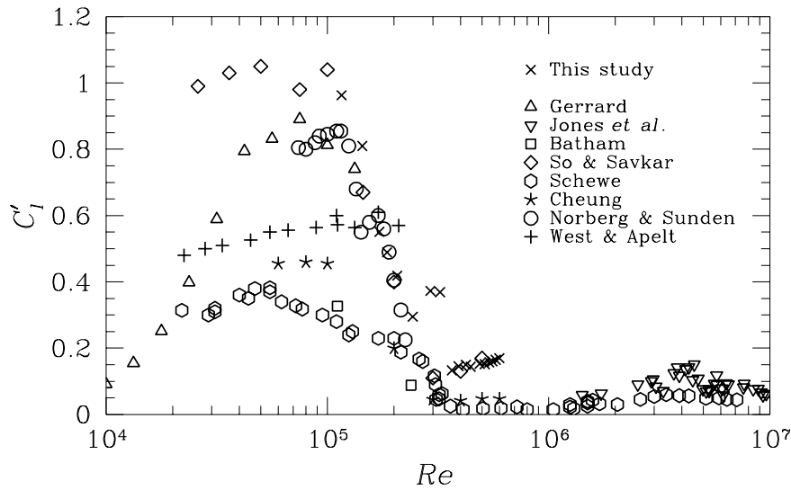
FIGURE 17. Published measurements of C_l' for nominally smooth flows, compared with those from this experimental programme.
