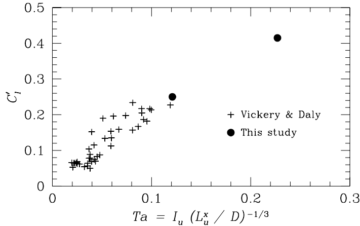
FIGURE 20. Estimates of sectional coefficients of lift C'_l and turbulence parameter Ta = I_u (L_u^x / D)^{-1/3} presented by Vickery and Daly (1984), together with values obtained at the upper end of the Reynolds number range ( Re \approx 5 \times 10^5 ) in the present experiments.
