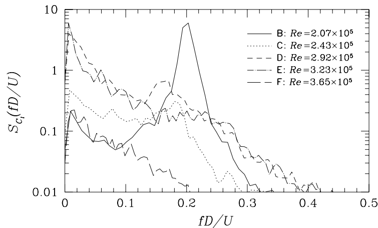
FIGURE 7. Smooth flow: changes in lift spectra during the transition B–F.
