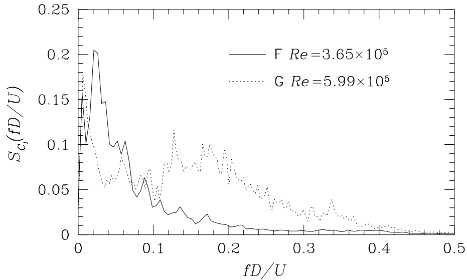
FIGURE 8. Spectra of lift force at points corresponding to F & G in fig. 5.
