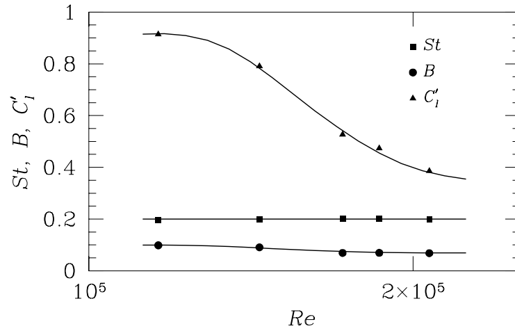
FIGURE 6. The spectral parameters Strouhal number ( St ), Bandwidth ( B ) and standard deviation of coefficient of lift ( C'_l ) fitted to the lift forces measured in smooth flow. Values are averages from the two central transducers.
