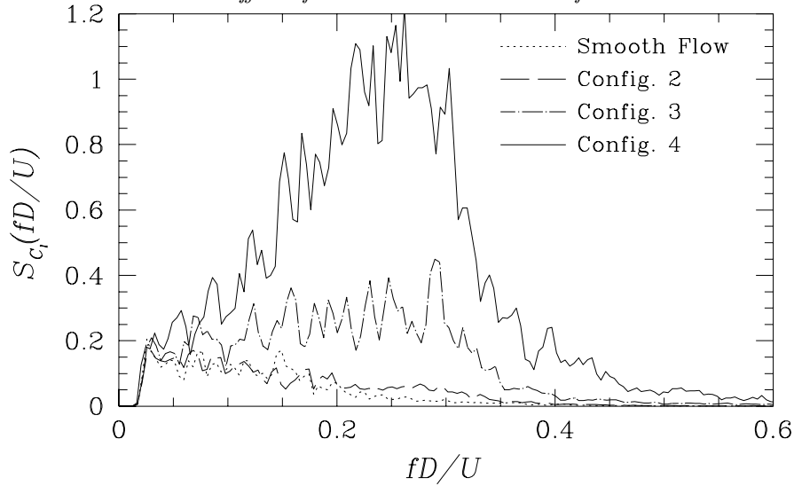
FIGURE 18. A comparison of lift force spectra recorded at transducer 4 at Reynolds numbers near 4.6 \times 10^5 in smooth and turbulent flows.
