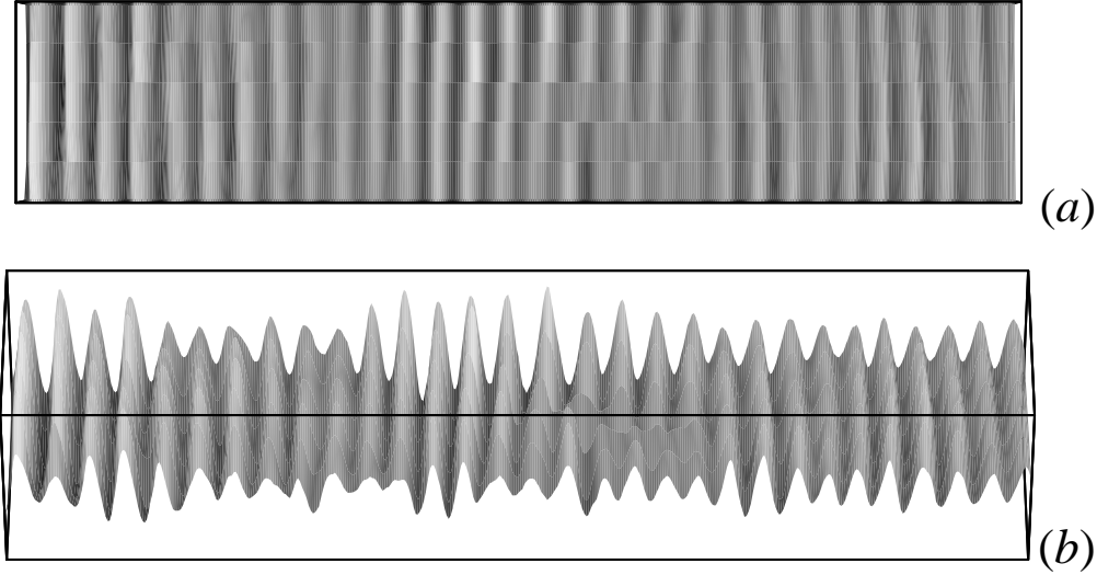
FIGURE 14. Visualized lift/time series surface for smooth subcritical flow ( Re = 1.6 \times 10^5 ). Approximately 30 vortex-shedding cycles are represented. (a); View from above surface (spanwise direction: up and down page; time coordinate: across page; coefficient of lift: normal to page). (b); Same surface, but with the viewpoint displaced in the spanwise direction.
