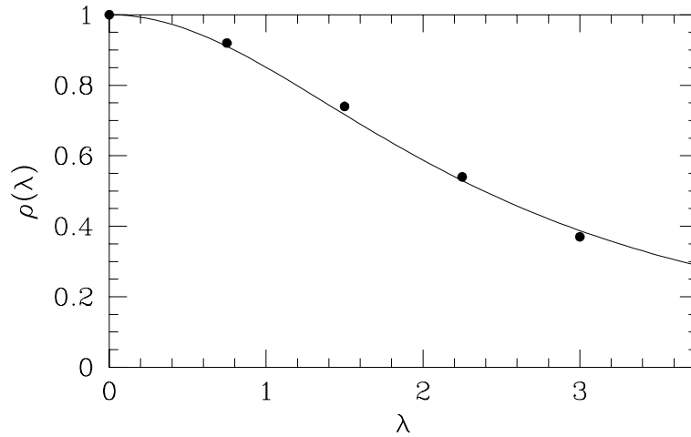
FIGURE 15. Spanwise distribution of the average correlation coefficient of lift force. Also shown is a fitted curve which provides a correlation length \Lambda of \sim 3.75 D .
