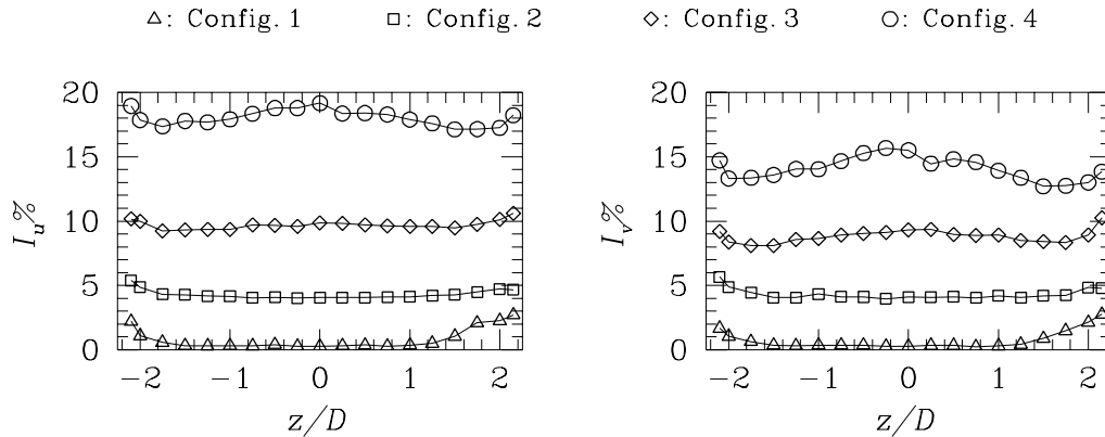
FIGURE 3. Distributions of longitudinal and transverse turbulence intensities ( I_u = u'/U & I_v = v'/U ) along cylinder axis position for the four flow configurations.
