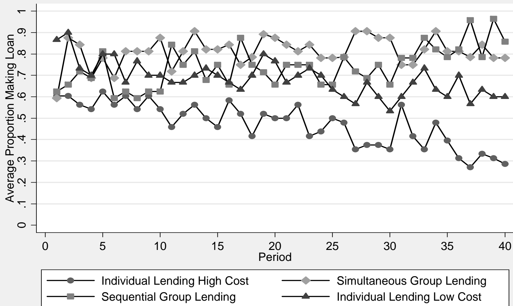
Figure 3: Average Proportion Making Loan, by treatment
