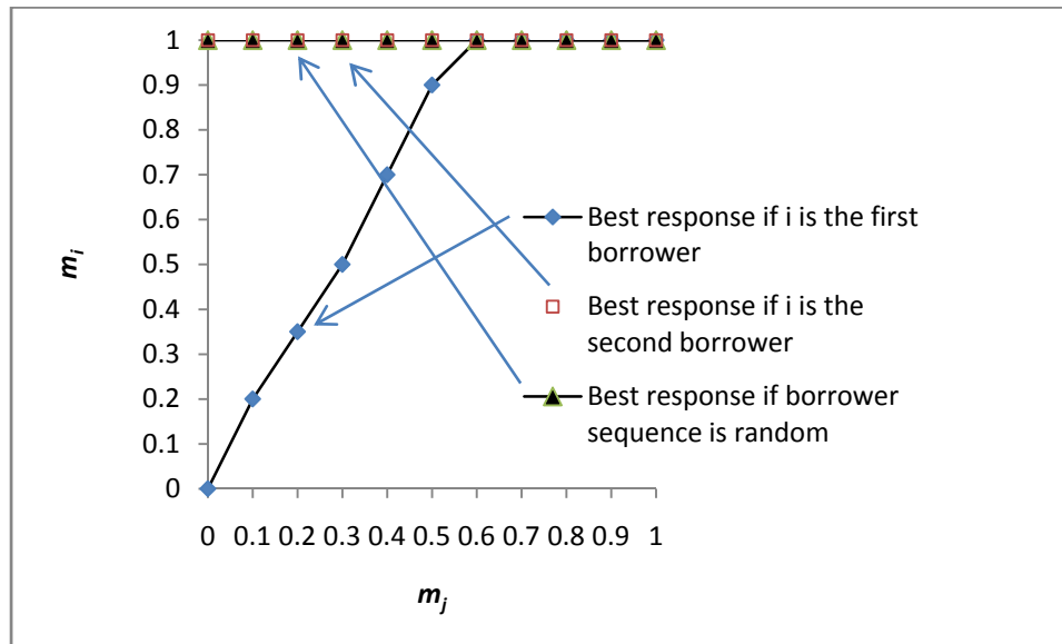
Figure 2: Reaction Functions of Borrower i in the Sequential Lending Treatment
