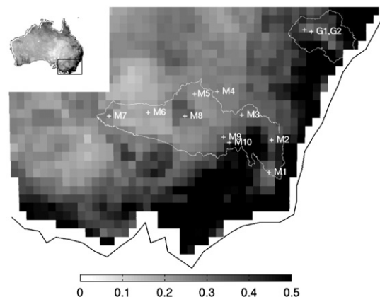
Fig. 2. Location of the Murrumbidgee and Goulburn Monitoring Network monitoring stations used in this study, overlaid on the mean 2006 NDVI. The NDVI has been aggregated to the (0.25°) AMSR-E grid. See Table 1 for explanation of station codes.
