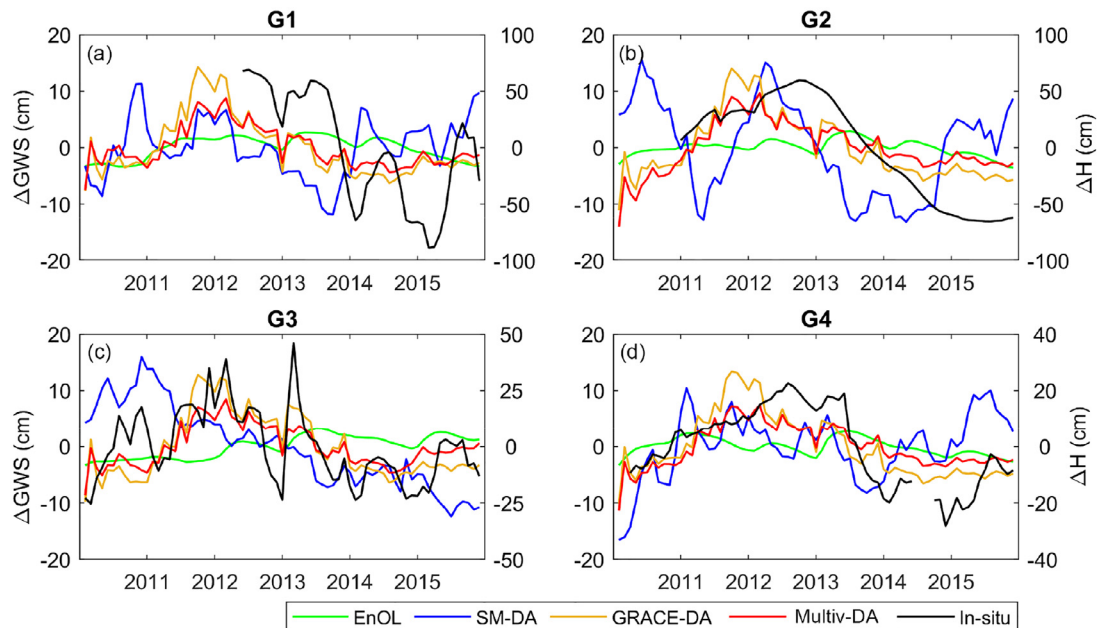
Fig. 10. The monthly groundwater storage variations ( \Delta GWS ) at G1 – G4 pixels computed from different DA approaches (SM DA, GRACE DA, and multivariate DA). The EnOL estimates and the in situ groundwater level variations ( \Delta H ) are also shown for comparison.
