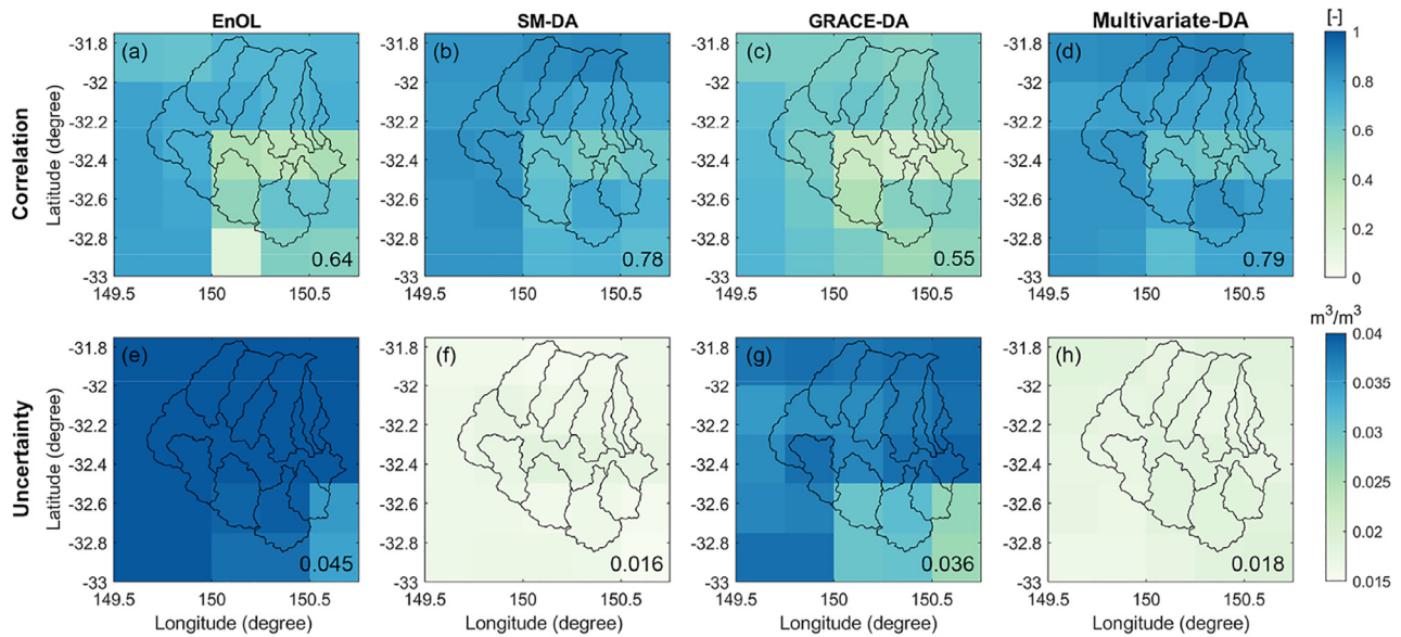
Fig. 3. The correlation coefficients (top row) and uncertainty (ensemble spread, bottom row) of the 0–5 soil moisture estimates computed between the SMOS data and different DA case studies. The averaged correlation and error values of the Goulburn catchment are given in each figure.
