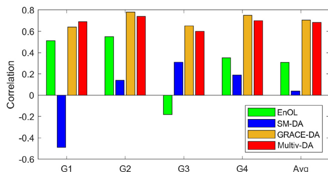
Fig. 11. The correlation coefficients of the \Delta GWS estimates at (a) G1, (b) G2, (c) G3, and (d) G4 pixels computed from EnOL and different DA case studies. The averaged correlation values (Avg) of G1 – G4 are also shown.
