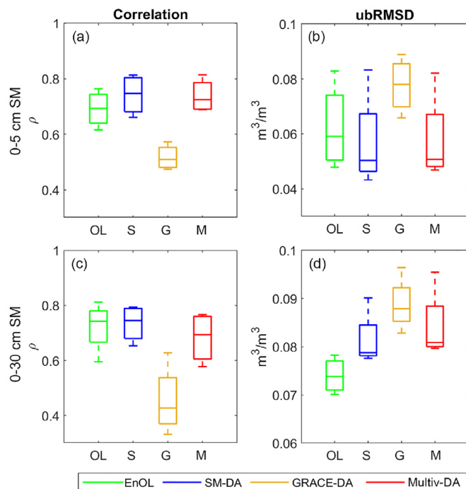
Fig. 8. The correlation coefficients (a, c) and unbiased root mean square differences (ubRMSD; b, d) of the 0 – 5 cm soil moisture (top row) and 0 – 30 cm soil moisture (bottom row) computed from the estimate of different DA case studies at S1 – S4 (S: SM DA, G: GRACE DA, M: Multivariate DA). The statistical results of the EnOL (OL) are also shown.
