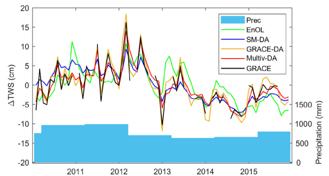
Fig. 5. The monthly basin-averaged \Delta TWS computed from different DA approaches (SM DA, GRACE DA, and multivariate DA). The EnOL estimate, the GRACE observation, and the yearly precipitation accumulated between April and May are also shown for comparison.
