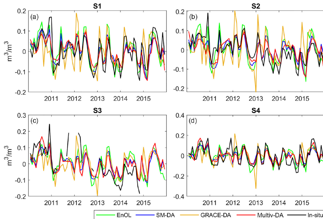
Fig. 7. The monthly “0 – 5 cm” soil moisture variations estimated at S1 – S4 pixels computed from different DA approaches (SM DA, GRACE DA, and multivariate DA). The EnOL estimates and the in situ soil moisture data are also shown for comparison.
