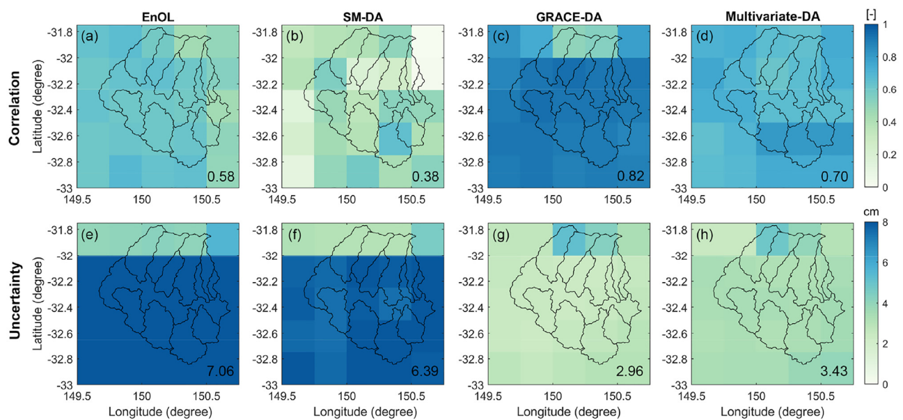
Fig. 6. The correlation coefficients (top row) and errors (ensemble spread, bottom row) of the \Delta TWS estimate computed between the GRACE observation and different DA case studies. The averaged correlation and error values of the Goulburn catchment are given in each figure.
