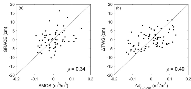
Fig. 4. Scatter plots between the basin-averaged \Delta TWS and soil moisture anomaly ((a) GRACE Vs. SMOS, and (b) CABLE-estimated \Delta TWS and \Delta\theta_{0-5cm} ) of the Goulburn catchment. The correlation coefficient ( \rho ) is provided in each figure.
