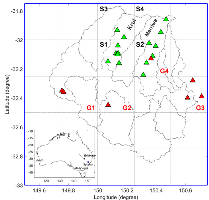
Fig. 1. The geographical location of the Goulburn River catchment, located in South-East Australia (see the inserted map). The black dotted squares indicate the 25 km model grid cells while the blue boundary denotes the GRACE grid cell used in this study. The locations of the in situ soil moisture and groundwater data are shown as green and red triangles, respectively. All in situ soil moisture data inside the same model grid cell are averaged, resulting in S1 – S4 in situ soil moisture grid cells. A similar approach is applied to the in situ groundwater data, resulting in G1 – G4 in situ groundwater grid cells. (For interpretation of the references to color in this figure legend, the reader is referred to the web version of this article.)
