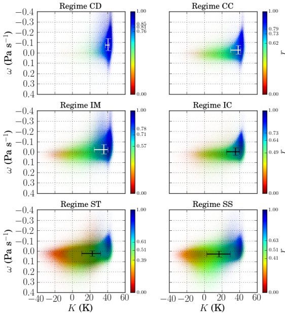
Figure 3: Scatter diagram of the relationship between modified K-index ( x -axis), vertical velocity ( y -axis) and saturation ratio (colour) for each regime. Quartile values are indicated by the crosses and colourbar ticks.
