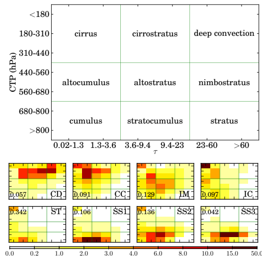
Figure 1: (Top) Cloud morphologies associated with the ISCCP joint-histogram (Rossow and Schiffer, 1999; Hahn et al., 2001). (Bottom) Joint-histograms of the centroids of the eight regimes (see Table 1). Numbers indicate their relative frequencies of occurrence (FOC) over the ocean.
