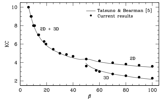
Figure 13: Transition results for both two and three-dimensional cases. Also shown are the corresponding regime boundaries of Tatsuno & Bearman [5].
