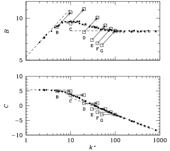
Figure 13: Nikuradse's data [6] for roughness function B and log-law correction constant C as functions of dimensionless sand roughness height k^+ . Data for the corrugated wall at Re_\tau = 314 are also shown (cf. figure 10), both in raw state, and corrected to an equivalent sand roughness height.
