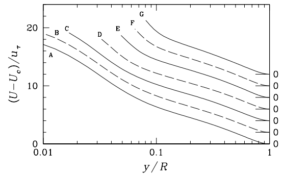
Figure 9: Normalised velocity defect (U - U_c)/u_\tau for different corrugation-heights h in turbulent flow, Re_\tau = 314 . Note that cases for different corrugation height are offset vertically of clarity. Cf. figure 5.
