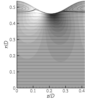
Figure 2: Streamlines and contours of pressure (dark grey represents low pressure) for laminar flow at Re_\tau = 78.6 , geometry case G. Since the flow is laminar and steady, only a single module of the wavy wall is represented in the laminar flow calculations.
