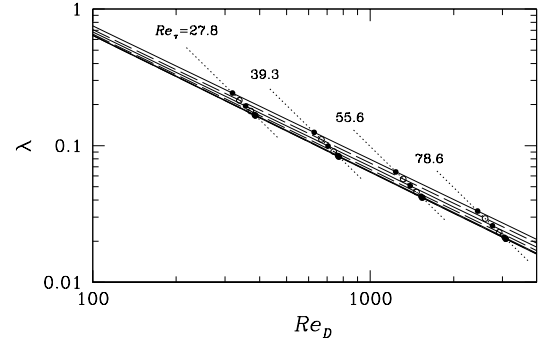
Figure 6: Pipe friction factor \lambda as a function of Re_D for laminar flows from four different values of Re_\tau . In each set, the lowest value of \lambda corresponds to the smooth pipe, case A (where \lambda = 64/Re_D ), the upper point to case G.
