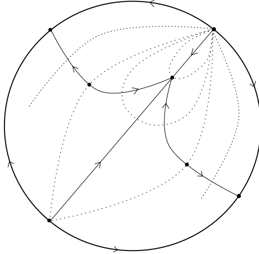
FIGURE 3. Plausible behavior on a periodic cs -leaf associated to a regular periodic point of the pseudo-Anosov. The dotted lines correspond to the strong stable manifolds.
