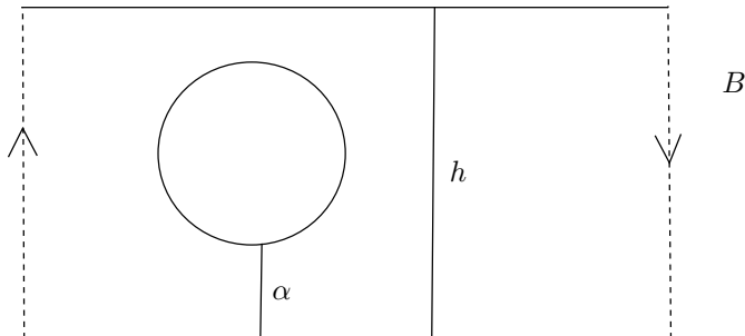
FIGURE 1. The surface B .
