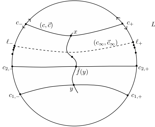
FIGURE 2. Depiction of the elements in the proof.
