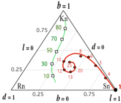
Figure 6. The red spiral on the right panel shows typical small group evolution, averaged over six small groups. The green curve shows the positions of 20 vertex random graphs with edge probabilities as indicated.
