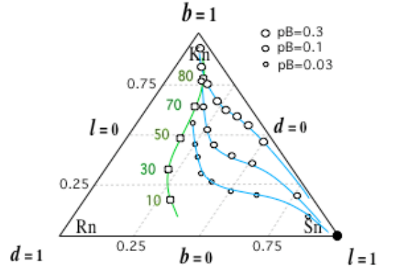
Figure 3. Three evolutionary trajectories (blue) show different probabilities of bonding (30% largest circles; 10% middle circles; 3% smallest circles) and constant member recruitment of 30%. The green locus shows the l, b, d values for 20 vertex Erdős-Rényi random graphs, with edge probabilities as indicated.
