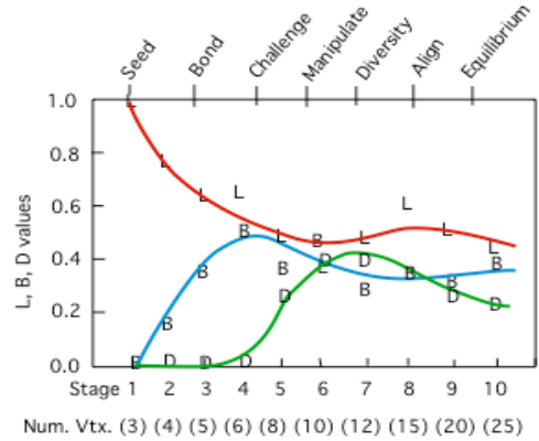
Figure 5. An example of how L, B, D vary in the evolution of a small group. The size of the group is shown on the bottom line.
