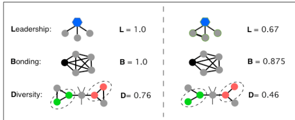
Figure 1. Subgraphs that capture the key properties of groups and their evolution. Left: Graphs with maximal or near-maximal values of the L , B , D parameters. Right: new L , B , D values when subgraphs at left are revised with one edge addition (top), with one deletion (middle), or with two deletions (bottom.)
