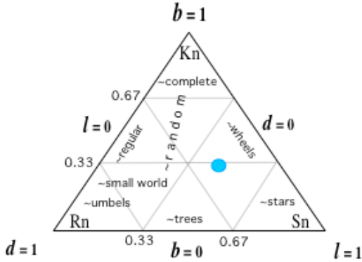
Figure 2. Regions of some familiar graphs are indicated on the projection of L, B, D onto the 1, 1, 1 plane. The blue circle indicates the terminal equilibrium location of evolving small groups.
