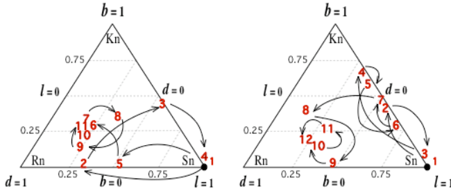
Figure 4. Loci of evolution from S_3 for two simulations, with values for pR, pB, pQ of 0.30, 0.30, 0.30 for the left panel, and 0.60, 0.30, 0.40 for the right panel. The behavior is very haphazard.
