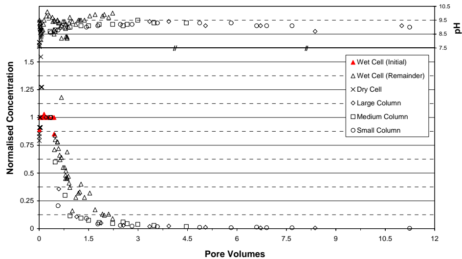
Figure 2. Leached ash – Salinity and pH versus pore volumes (Mudd et al , 2004)
