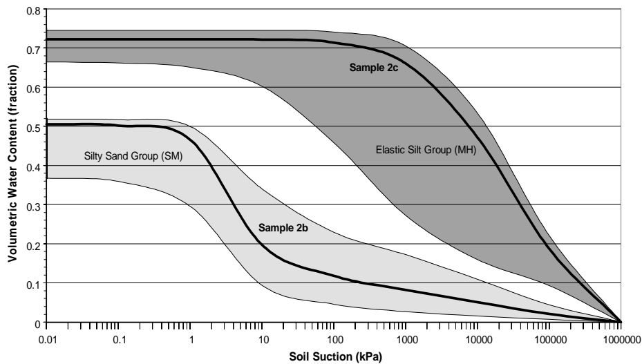
Figure 1. General range for soil water characteristic curves of Loy Yang leached ash samples
