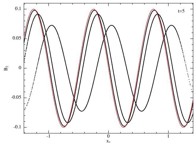
Figure 26. Results of the 3D circularly polarised Alfvén wave test after 5 periods, showing perpendicular component of the magnetic field on all particles (black dots) as a function of distance along the axis parallel to the wave vector. Results are shown using 32 \times 18 \times 18 , 64 \times 36 \times 39 and 128 \times 74 \times 78 particles (most to least damped, respectively), compared to the exact solution given by the solid red line. Convergence is shown in Figure 27.
