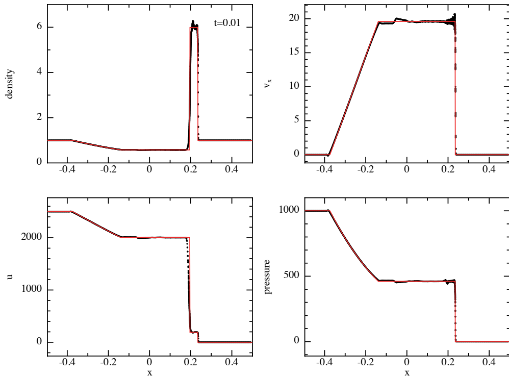
Figure 11. As in Figure 10 but with code defaults for dissipation switches ( \alpha^{\text{AV}} \in [0, 1] ; \alpha_u = 1 ). As in Figure 9 the velocity field behind the shock is more noisy with switches applied, but the switches reduce the numerical dissipation away from shocks.
