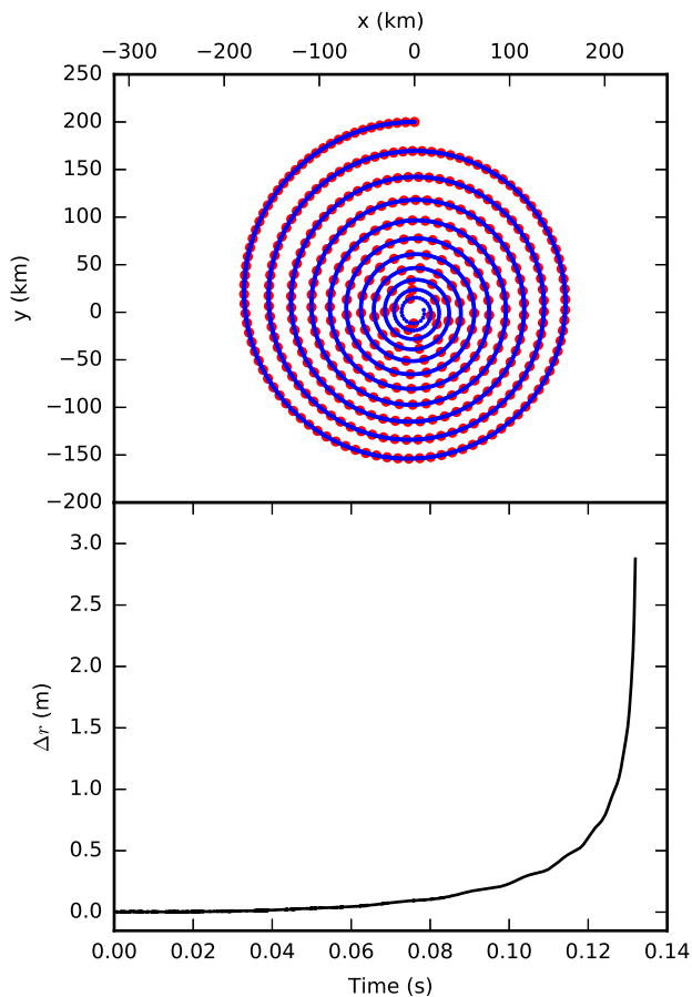
Figure 18. Inspirals of a test particle subjected to Poynting-Robertson drag using PHANTOM (blue curve) compared to the expected solution (red curve). For clarity, only some of the points are plotted. The results are indistinguishable on this scale. Bottom panel shows the distance ( \Delta r ) between the PHANTOM particle and the test code particle. This demonstrates that the implementation of Poynting-Robertson drag in PHANTOM is consistent with a 4th order numerical solution to (106).
