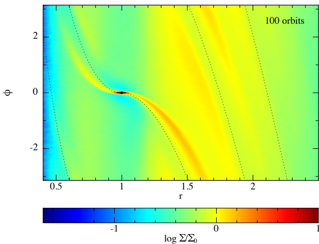
Figure 22. Planet-disc interaction in 3D, showing the ‘viscous Jupiter’ calculation comparable to the 2D results shown with various grid and SPH codes in Figure 10 of de Val-Borro et al. (2006). The dotted lines show the estimated position of the planetary shocks from Ogilvie & Lubow 2002. The offset between this solution and the numerical shock position is due to the approximate nature of the analytic solution (see de Val-Borro et al. 2006).
