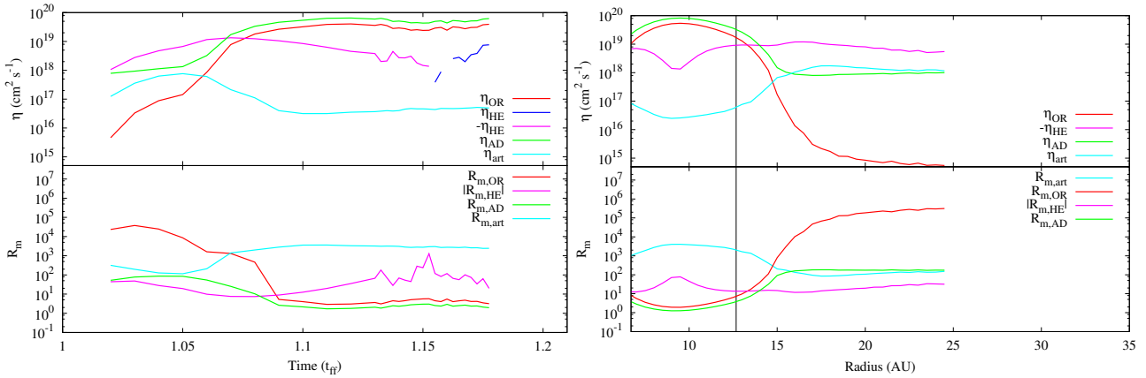
Figure 12. Non-ideal MHD coefficients, \eta (top panels) and magnetic Reynolds numbers, R_m = v_c r / \eta (bottom panels) for the non-ideal MHD model with \mu_0 = 5 and \mathbf{B}_0 \cdot \boldsymbol{\Omega}_0 < 0 . The left-hand panel shows the average values in the disc, and the right-hand panel shows the radial profile at t = 1.12 t_{\text{ff}} . Horizontal axes are chosen for consistency with other plots in this paper. The vertical line in the right-hand panel corresponds to the defined radius of the disc at that time. Shortly after the formation of the disc, the Hall effect is the dominant term, but as the disc begins to dissipate, the dissipative terms begin to dominate. The value of R_m \gtrsim 1 indicates that the diffusion terms are important in the disc.
