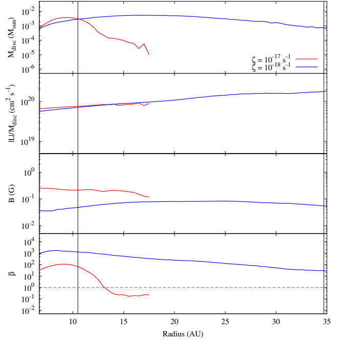
Figure 17. As in Fig. 14, but for two different cosmic ray ionisation rates, \zeta , for the non-ideal MHD model with \mu_0 = 5 and \mathbf{B}_0 \cdot \boldsymbol{\Omega}_0 < 0 . The vertical lines at r \approx 11 and 35 \text{ AU} represent the defined radii of the discs using \zeta = 10^{-17} and 10^{-18} \text{ s}^{-1} , respectively.
