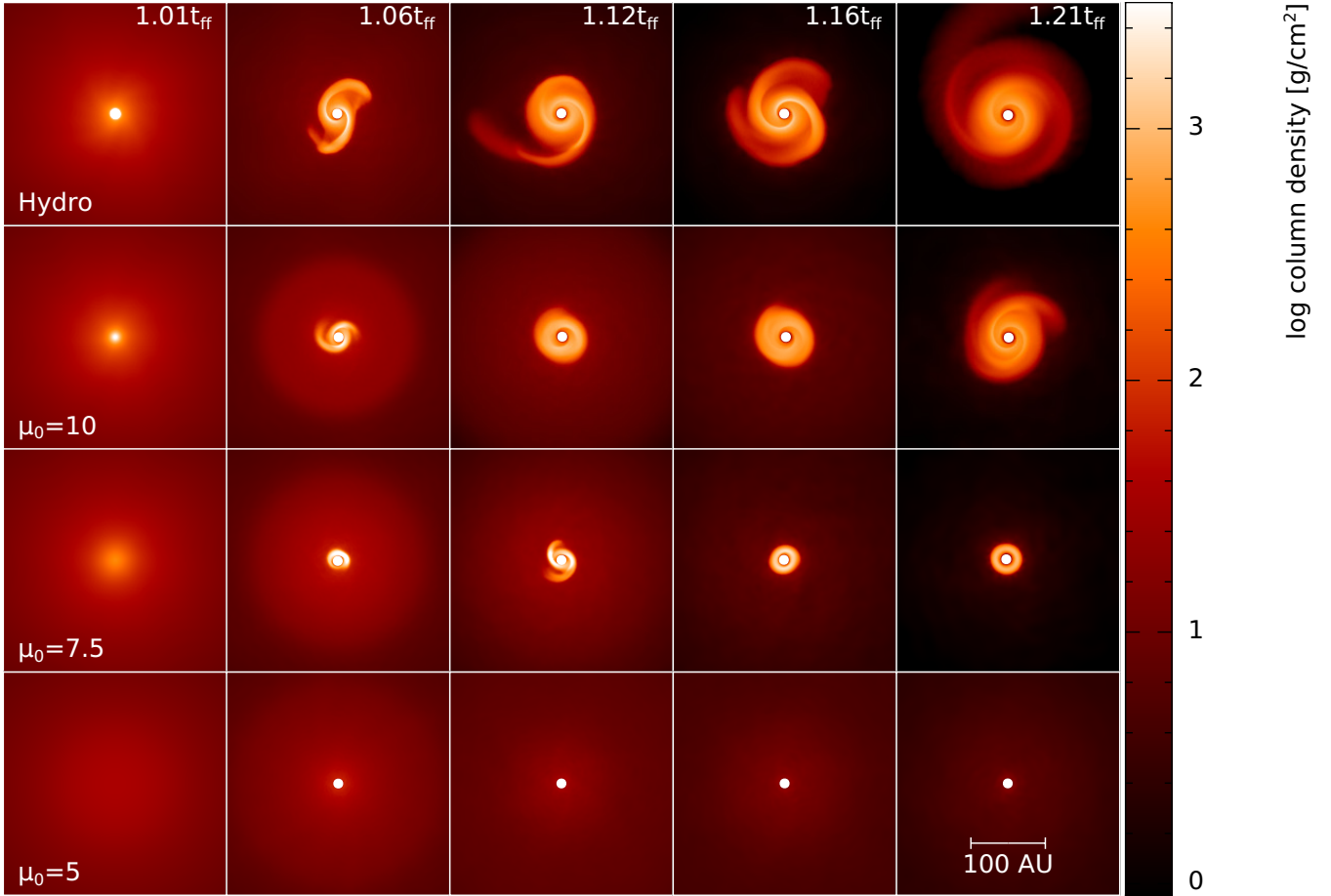
Figure 2. Face-on gas column density using ideal MHD. The initial rotation is counter-clockwise and the initial magnetic field is directed out of the page (i.e. \mathbf{B}_0 \cdot \boldsymbol{\Omega}_0 > 0 ). Each model is initialised with \sim 3 \times 10^5 particles within the sphere. From left to right, the columns represent snapshots at a given time (in units of the free-fall time, t_{\text{ff}} = 2.4 \times 10^4 yr). The rows represent models with different initial magnetic field strengths given in terms of \mu_0 (i.e. the initial mass-to-flux ratio normalised to the critical mass-to-flux ratio). The top row has no initial magnetic field and the bottom row has the strongest magnetic field (i.e. increasing magnetic field strength corresponds to a decreasing value of \mu_0 ). The white circles represent the sink particle with the radius of the circle representing the accretion radius of the sink particle. Each frame is (300 \text{ AU})^2 . The discs grow in size and mass with time. At any given time, the models with stronger magnetic fields have smaller and less massive discs than the models with the weaker initial magnetic field. The hydrodynamic model yields the largest and most massive disc in our entire suite of simulations.
