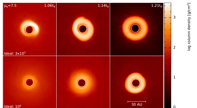
Figure 4. Face-on column density as in Fig. 2 but for ideal MHD at two different resolutions and zoomed in to (90 \text{ AU})^2 ; both use \mu_0 = 7.5 . The open circles represent the sink particle with the radius of the circle representing the accretion radius of the sink particle. At both resolutions, disc masses and radii are similar.
