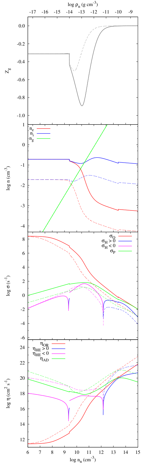
Figure 1. Top to bottom: Grain charge, charged species number densities, conductivities and resistivity coefficients, using \zeta = 10^{-17} (solid lines) and 10^{-18} s^{-1} (dashed lines). The top ticks on each panel correspond to mass density (top scale), and the bottom ticks correspond to number density (bottom scale). The discontinuities at \rho_n = 10^{-14} and 10^{-10} g\ cm^{-3} correspond to the discontinuities in temperature caused by the assumed equation of state.
