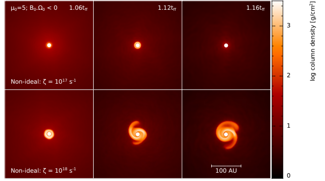
Figure 16. As in Fig. 2, but for two different cosmic ray ionisation rates, \zeta , for the non-ideal MHD model with \mu_0 = 5 , \mathbf{B}_0 \cdot \boldsymbol{\Omega}_0 < 0 , and \sim 3 \times 10^5 particles initially in the sphere. For this model, decreasing \zeta allows a large disc to form and persist for the duration of the simulation; for the larger value of \zeta , the disc dissipates by t \approx 1.15t_{\text{ff}} .
