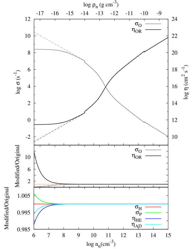
Figure B1. Top: Ohmic conductivity and resistivity, using the modified Hall parameters used in all calculations (solid) and the original Hall parameters (dashed). In all cases, \zeta = 10^{-17} \text{ s}^{-1} . The vertical range is different than in Figs. 1 and A2 to avoid truncating the curves. Middle and bottom: Ratios of the conductivities and resistivities calculated using the modified Hall parameters to that using the original Hall parameters. Note that the bottom two panels have different vertical scales from one another. The top ticks on each panel correspond to mass density (top scale), and the bottom ticks correspond to number density (bottom scale). At the lower end of the given number density range, Ohmic conductivity and resistivity differ significantly depending on the Hall parameters; the remaining conductivities and resistivities are relatively unaffected by the form of the Hall parameters. At the densities where the choice of the Hall parameter affects the Ohmic conductivity and resistivity, Ohmic resistivity is the weakest non-ideal MHD effect by at least seven orders of magnitude.
