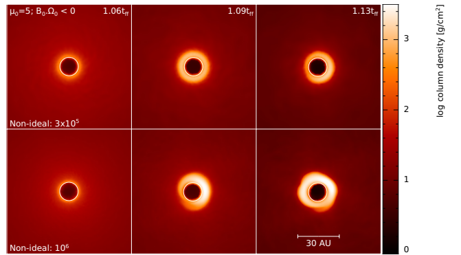
Figure 7. Resolution study, as in Fig. 4, but for non-ideal MHD with \mu_0 = 5 and \mathbf{B}_0 \cdot \boldsymbol{\Omega}_0 < 0 . For non-ideal MHD, increasing the resolution decreases the mass of the star+disc system by only \sim 5 per cent.
