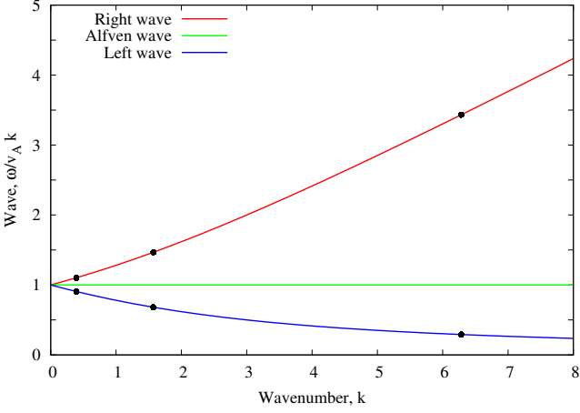
Figure C1. Dispersion relation for the left- and right-circularly polarised wave, corresponding to \eta_{\text{HE}} < 0 and > 0 , respectively. The solid circles are the numerically calculated phase velocities.
