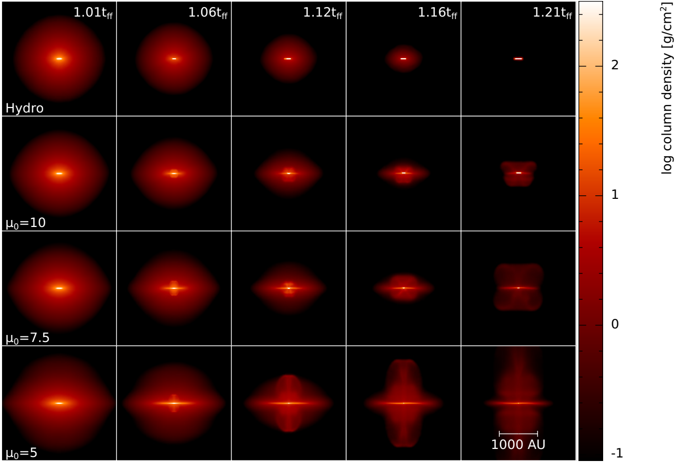
Figure 5. Edge-on gas column density using ideal MHD and zoomed out to (3000 \text{ AU})^2 and using a density range shifted down by a factor of ten to visualise the full extent of the outflows launched shortly after the collapse ( t \approx 1.02t_{\text{ff}} ) in the magnetic models. The models with stronger magnetic fields have faster and more collimated outflows.
