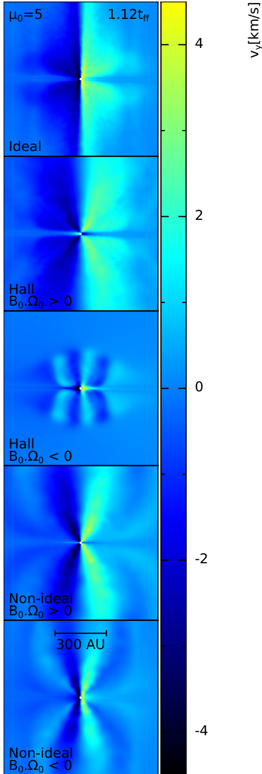
Figure 15. The velocity perpendicular to a slice through the outflow (i.e. v_y ) for five models with \mu_0 = 5 at t = 1.12t_{\text{ff}} . Each frame is (900 \text{ AU})^2 , which is smaller than in Fig. 11 so that details around the first hydrostatic core can be seen. The Hall-only model the \mathbf{B}_0 \cdot \boldsymbol{\Omega}_0 < 0 has a weak bipolar outflow, but forms a counter-rotating envelope. A weak counter-rotating envelope also exists in the non-ideal MHD model with \mathbf{B}_0 \cdot \boldsymbol{\Omega}_0 < 0 . None of the other models develop a counter-rotating envelope. The Ohmic-only and ambipolar-only models are very similar to the ideal and non-ideal MHD ( \mathbf{B}_0 \cdot \boldsymbol{\Omega}_0 > 0 ) models, respectively.
