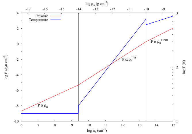
Figure A1. Pressure (red) and temperature (blue) resulting from the barotropic equation of state (Eqn. 5). The vertical lines are the threshold densities, \rho_d and \rho_c . The pressure is a continuous function of density, while temperature is discontinuous at the threshold densities.
