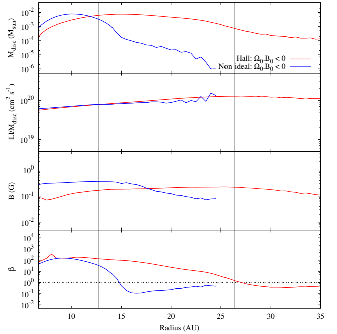
Figure 14. Radial profile of the disc at t = 1.12t_{\text{ff}} for the Hall-only (red) and non-ideal MHD (blue) models with \mathbf{B}_0 \cdot \boldsymbol{\Omega}_0 < 0 , for \mu_0 = 5 and \sim 10^6 particles. The profile includes all the gas particles with density \rho > \rho_{\text{disc,min}} , and starts at r = 6.7 \text{ AU} , which is the sink radius. The vertical lines at \sim 13 and 26 \text{ AU} represent the defined radii of the discs in the non-ideal MHD and Hall-only models, respectively. From top to bottom: Disc mass, specific angular momentum, magnetic field strength, and plasma beta.
