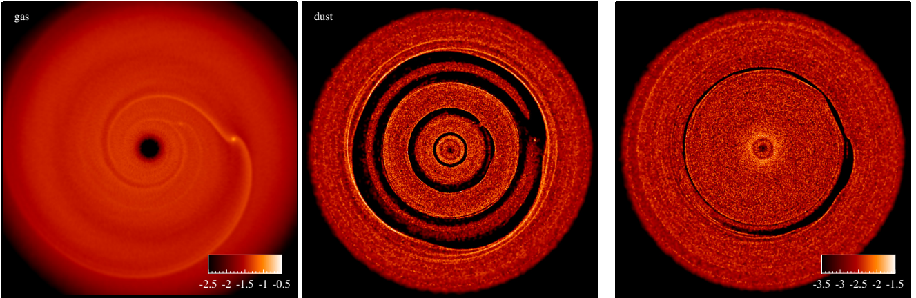
Figure 5. Similar to Fig. 1, but with a disc hosting three planets of mass 0.08, 0.1 and 0.52 M_J initially located at the same distance as the gaps detected in HL Tau. The first two planets open dust gaps according to Mechanism I, whereas the third planet is at the transition between the two mechanisms. Importantly, the tidal torque in the dust can not be neglected.
