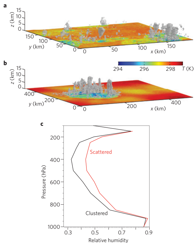
Figure 4 | What role does convective aggregation play in climate? In models, convective organization can exhibit a random distribution ( a ) or evolve spontaneously towards an aggregated state ( b ) 42 , increasingly so with increasing temperature 40 . c , In observations (relative humidity profiles from AIRS satellite measurements), the middle troposphere is drier in an atmosphere in which the same amount of precipitation is concentrated in a smaller number of convective clusters 39 . Figure reproduced with permission from a,b , ref. 42, AMS; c , ref. 39, AMS.
